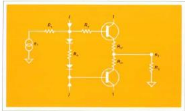
Fig. 4. Typical emitter follower Class-B stage.
