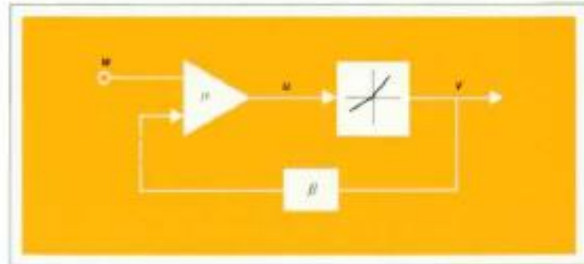
Fig. 3. Feedback amplifier incorporating nonlinear element.
