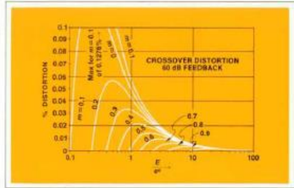
Fig. 13. Crossover distortion, 60 dB feedback.
