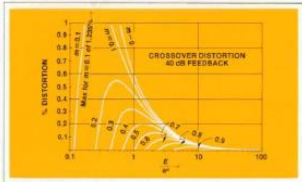
Fig. 12. Crossover distortion, 40 dB feedback.
