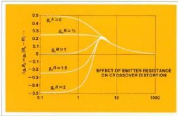
Fig. 6. Effect of emitter resistance on crossover distortion.
