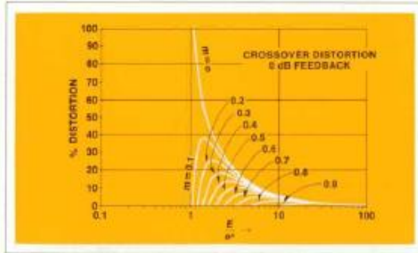
Fig. 10. Crossover distortion, 0 dB feedback.
