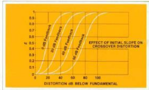
Fig. 14. Effect of initial slope on crossover distortion.
