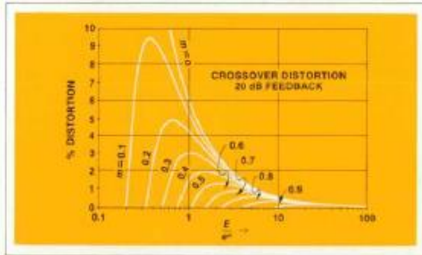
Fig. 11. Crossover distortion, 20 dB feedback.
