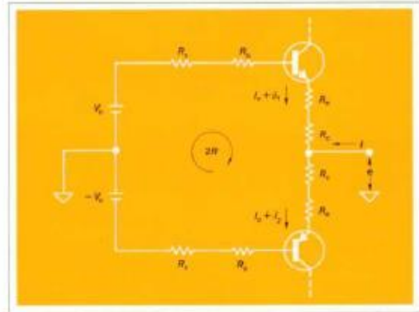
Fig. 5. To find optimum R_i , input is grounded, voltage applied to output.
